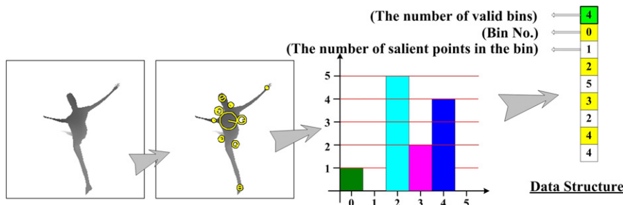
Fig. 6. Represent a depth-buffer view as a word histogram by the vector quantization of its SIFT local features.
