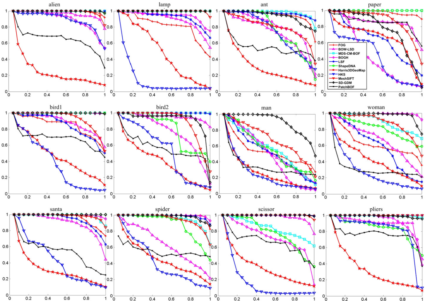
Fig. 16. Precision–recall curves of 11 methods evaluated for 12 different classes, respectively.
