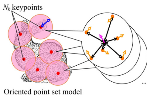
Fig. 8. Localized statistical features (LSF).
