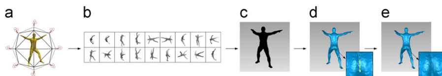
Fig. 4. Creating the watertight manifold for a 3D mesh. We first normalize the original model (a) so that it is located inside a unit geodesic sphere, and then a set of depth-buffer views (b) of the 3D mesh are captured on the 18 vertices of the bounding sphere. Afterwards, we convert those depth-buffer images into a point cloud (c), which is then utilized to generate a polygonal mesh (d). Finally, by fixing holes and other errors on the surface (d), we obtain a watertight manifold (e) without inner structures.
