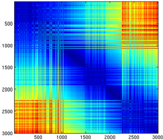
Fig. 11. The normalized geodesic distance matrix of the preprocessed snake model, which was shown in Fig. 10(a).
