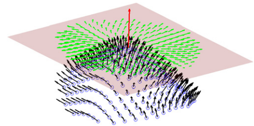
Fig. 12. The neighborhood of a scale space extremum with normals and projected normals.
