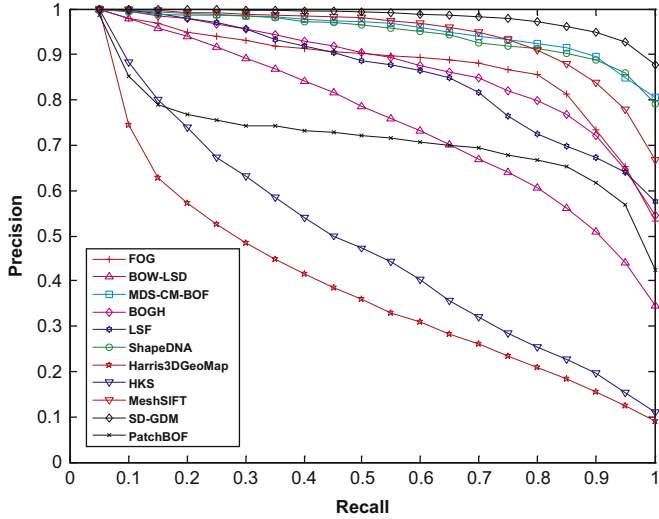
Fig. 15. Precision–recall curves of 11 methods evaluated for the whole database.
