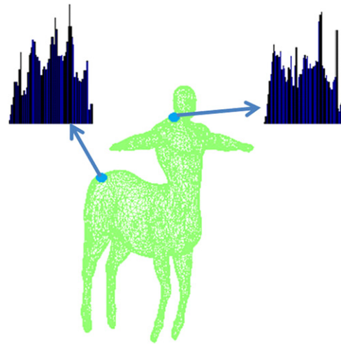
Fig. 7. Illustration for the histogram of geodesic distances computed at two points on the centaur model.
