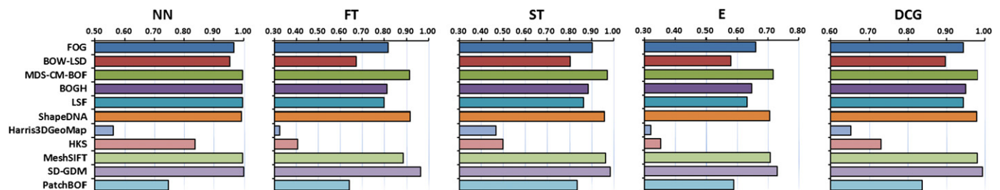
Fig. 14. Bar charts of the retrieval accuracies of 11 methods evaluated on the whole database using five standard measures, respectively.
