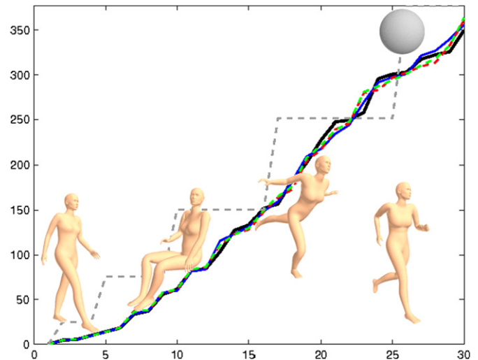
Fig. 9. First 30 eigenvalues plotted for the girl in four different postures as opposed to the spectrum of the sphere (gray) with same surface area (the position of the shapes in the plot is irrelevant).
